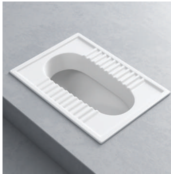
ORISSA 23" - 14ORI-23 Squatting Pan L430_D610_H310mm
