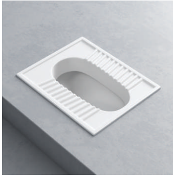
ORISSA 20" - 14ORI-20 Squatting Pan L400_D500_H250mm
